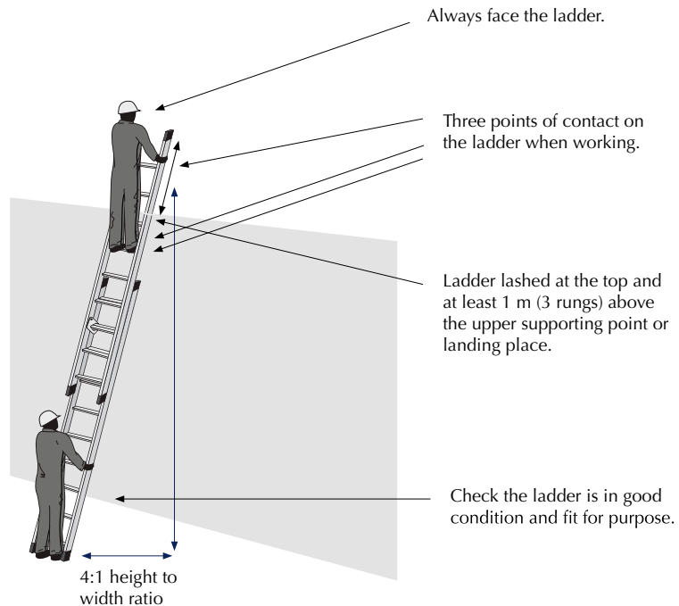
Figure 17.1 Portable ladder
