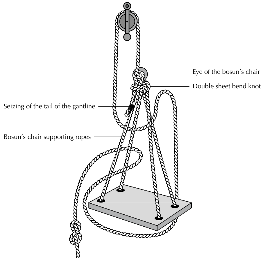
Figure 17.2 Bosun's chair
